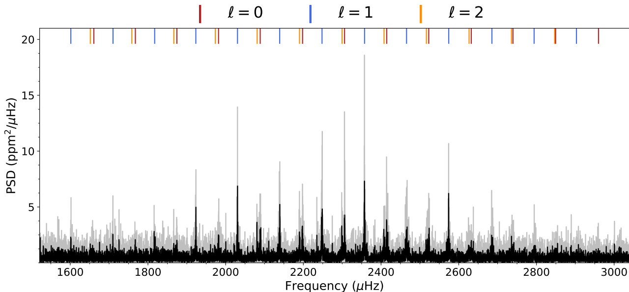
Fig. 6: The power spectral density of \chi Dra A for 20-s cadence observations is shown in light grey, along with an Epanechnikov filter (Epanechnikov 1969) of \Delta\nu/15 shown in black. The measured \ell = 0, 1 , and 2 modes from pipeline 1 (see Table C.1) are shown as red, blue, and orange lines on the top, respectively.
